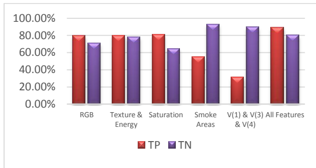
Figure 2: True positive and True negative classification results of different feature subsets
