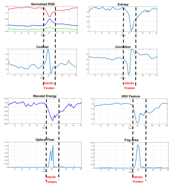
Figure 1: Extracted 10 features from 100 frames with smoke annotation.
