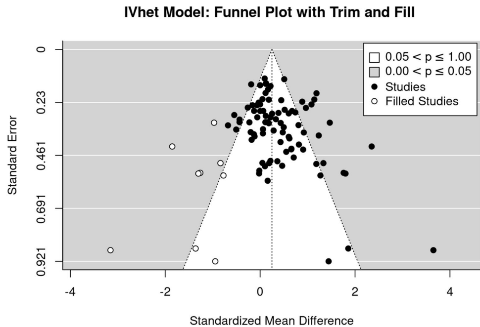
Fig. 3 Funnel plot with trim and fill on the effect of exercise on BMD at the lumbar spine
