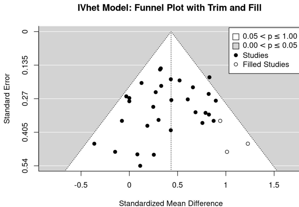
Fig. 7 Funnel plot with trim and fill on the effect of exercise on BMD at the total hip ROI
