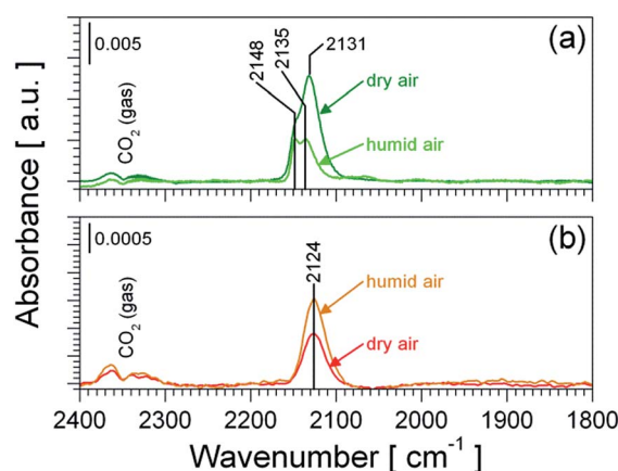
Fig. 7 Operando DRIFT spectra of \text{Pt:SnO}_2 PI (a) and \text{Pt:SnO}_2 GI (b) recorded during the exposure of 100 ppm CO in dry air (reference: dry air) and humid air (reference: humid air) at 300 °C. The spectra shown in (b) are based on the experimental data previously published by K. Großmann et al. 13
