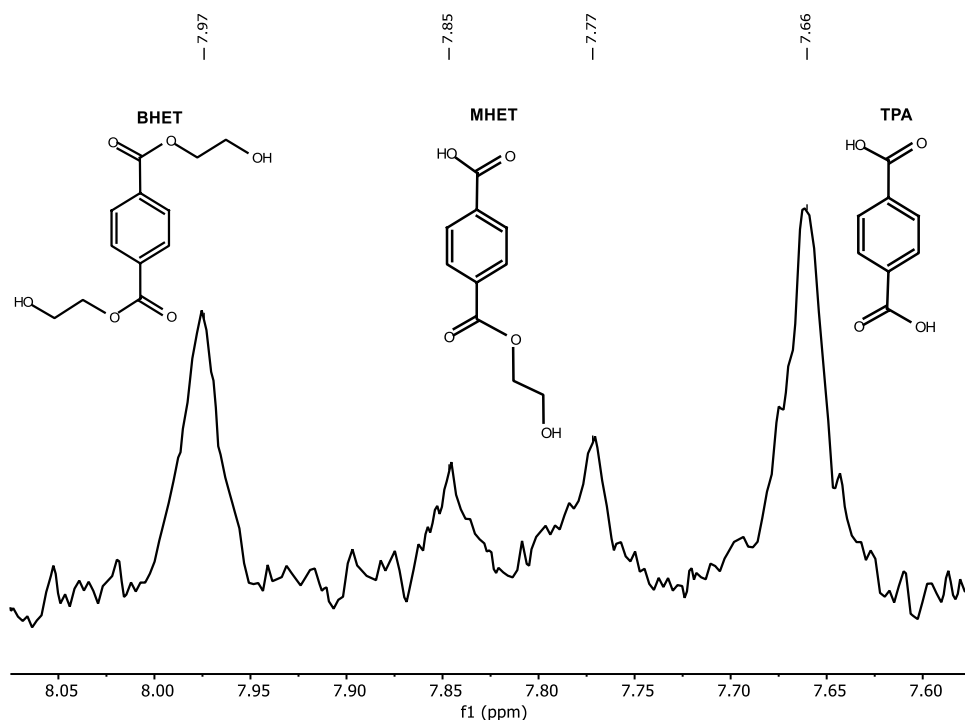
Fig. 1 Differentiation of the degradation products to confirm the suitability of ^1\text{H} NMR analysis. A mixture of 500\ \mu\text{M} of each product in buffer with pH 9 was analysed on a Spinsolve 60 Carbon Benchtop NMR spectrometer for 10 min. The abscissa shows the chemical shifts of the peaks. A singlet at 7.66 ppm indicates TPA, a doublet at 7.77 and 7.85 ppm indicates MHET, and a singlet at 7.97 ppm belongs to BHET. The degradation products could be clearly distinguished from each other
