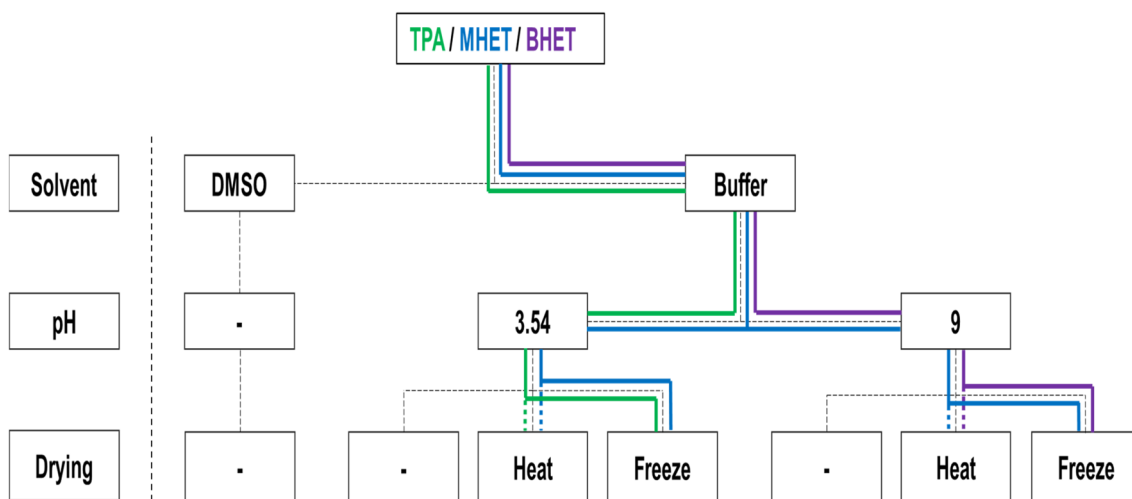
Fig. 2 Optimization strategy for absorption and ^1\text{H} NMR measurements. Different solvents, pH values and drying processes were investigated to determine the optimum conditions for the measurement of the degradation products, shown in coloured lines. The best results for TPA and MHET were achieved in buffer pH 3.54 after freeze-dry-
