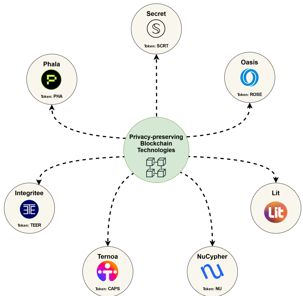
Figure 1. Privacy-preserving blockchains.
